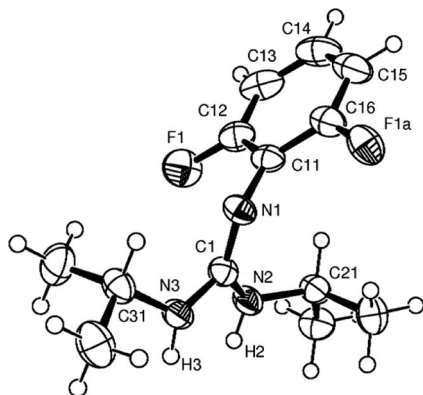
Figure 1. ORTEP representation (50%) of [(2\text{-FC}_6\text{H}_5)\text{N}]_2\text{C}\{\text{NH}i\text{Pr}\}_2 . Selected bond lengths [Å] and angles [°]. C(1)–N(1) 1.306(2), C(1)–N(2) 1.364(3), C(1)–N(3) 1.363(3), N(1)–C(1)–N(3) 118.73(19), N(1)–C(1)–N(2) 127.06(19), N(3)–C(1)–N(2) 114.15(18). Disordered fluorine atoms modelled over two sites.
